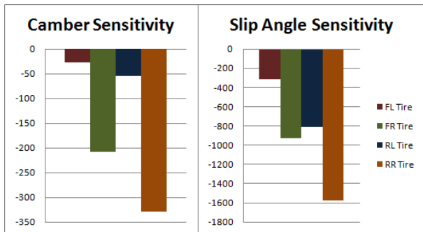
Figure 4: Camber sensitivity and slip angle sensitivity of lateral force for all four tires at the apex of a corner
