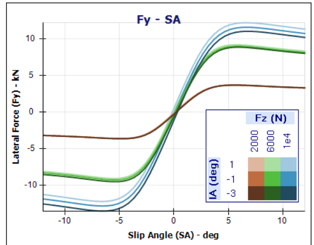
Figure 1: Lateral force characteristics for the tire used in this example
