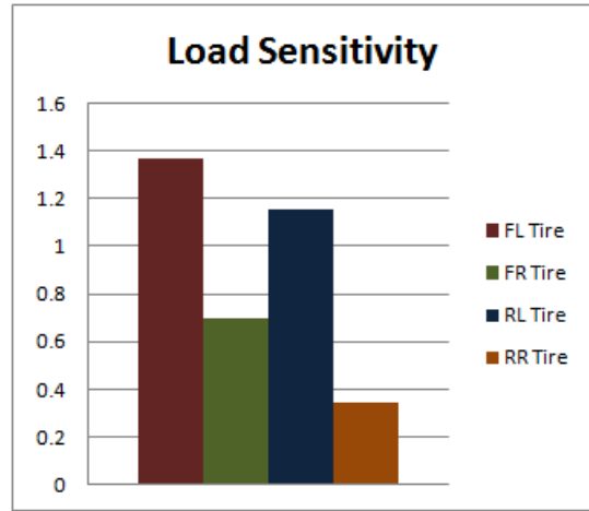
Figure 6: Load sensitivity of the four tires at the apex of a corner
