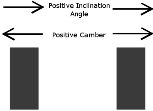
Figure 5: Rear view of car showing camber and inclination angle for the ISO tire coordinate system.
