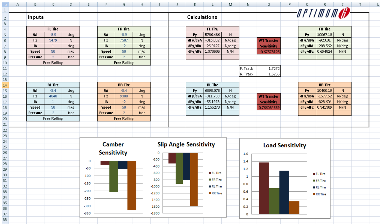
Figure 3: The spreadsheet using the OptimumT Add-in
